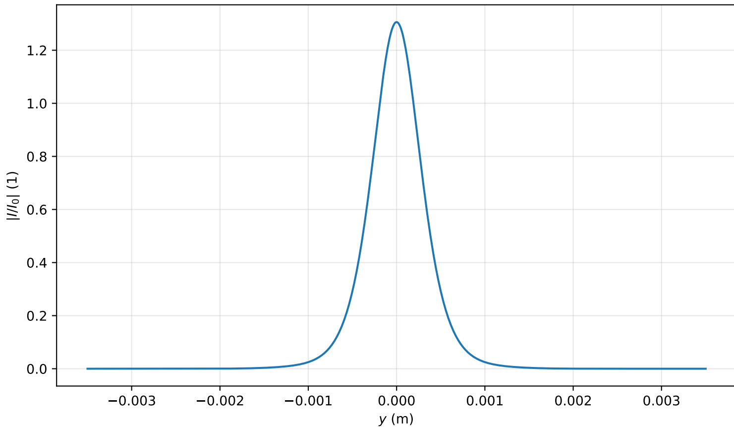
Intensity profile I(x = 0, y, z = 2.070)/I_0 , P_{in}=0.8P_{cr} , artificial time
